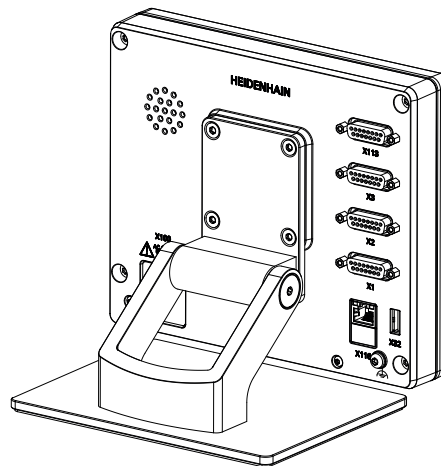
Multi-Pos stand (example: ND 7013)
