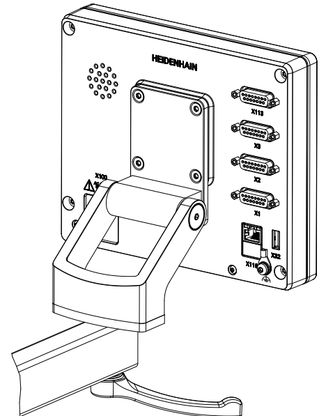
Multi-Pos holder on mounting arm (example: ND 7013)
